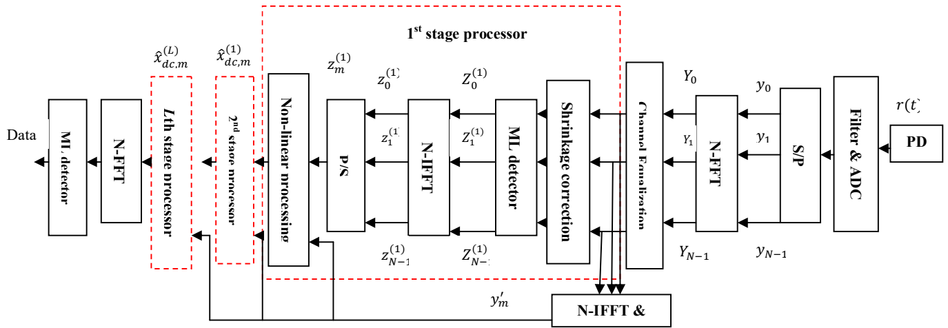
Fig. 6. Multiple stage non-linear processing receiver.
