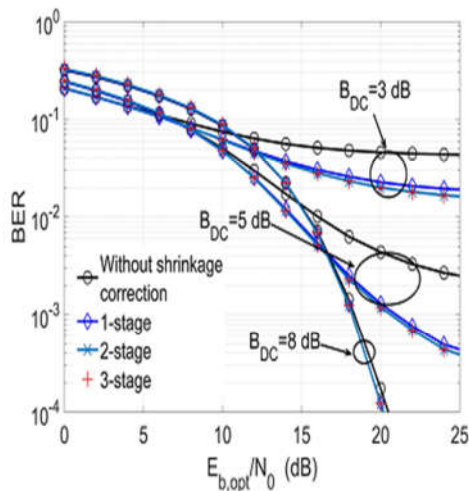
Fig.7. BER performance using multiple stage clipping noise mitigation processor (16-QAM).
