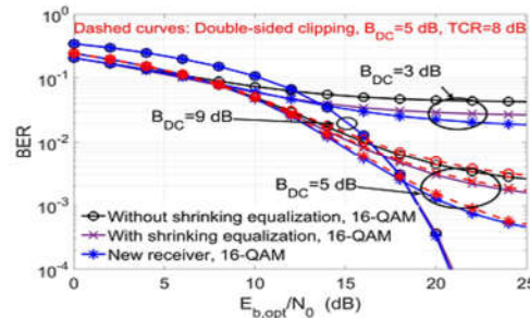
Fig.5. Comparison between conventional receivers (with and without shrinkage correction) and clipping noise mitigation receiver using 16-QAM.
