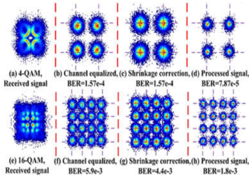
Fig.9. Experimental results of the signal constellation.
