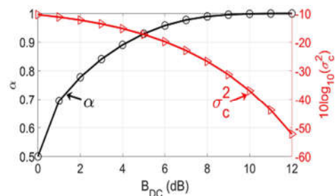
Fig.2. Attenuation and clipping noise variance versus dc bias level (dB).
