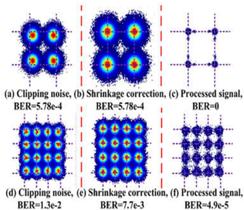
Fig.3. Signal constellation: (a) 4-QAM, after clipping, (b) 4-QAM, after shrinkage correction, (c) 4-QAM, after clipping noise mitigation, (d) 16-QAM, after clipping operation, (e) 16-QAM, after shrinkage correction, (f) 16-QAM, after clipping noise mitigation.
