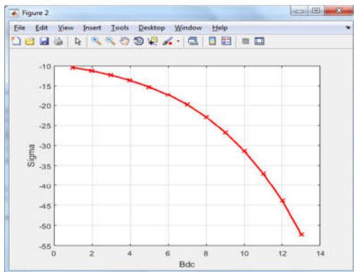
Fig.2. Clipping noise variance versus bias level (dB).
