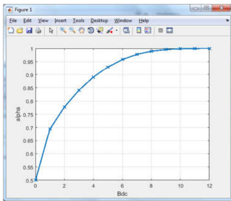
Fig.1. Attenuation versus bias level (dB).
