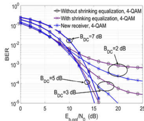
Fig.4. Comparison between conventional receivers (with and without shrinkage correction) and clipping noise mitigation receiver using 4-QAM.
