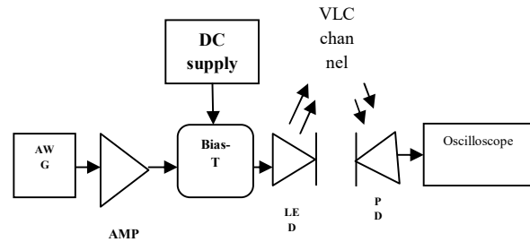
Fig.8. Experimental setup.
