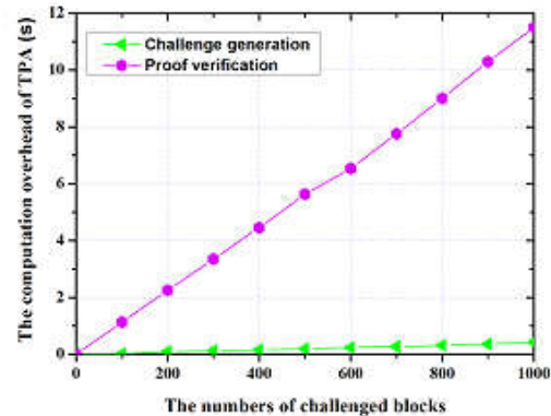
Fig.2. The computation overhead of the TPA in the phase of integrity auditing.
