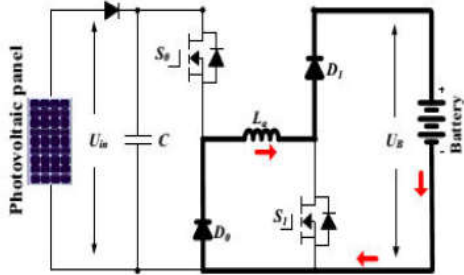
(b) Battery charging
