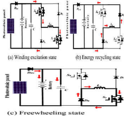
Fig7: Working states at mode 2
