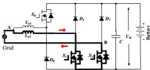
(a) Grid charging state 1 (Ugrid>0)
