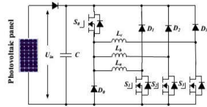
(c) Operation circuit under mode 3
