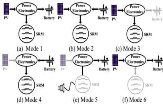
Fig3: Six operation modes of the proposed Triport topology
