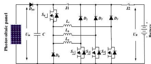
Fig2: the proposed Tri-port topology for PV-powered SRM drives.
