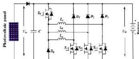
(b) Operation circuit under mode 2
