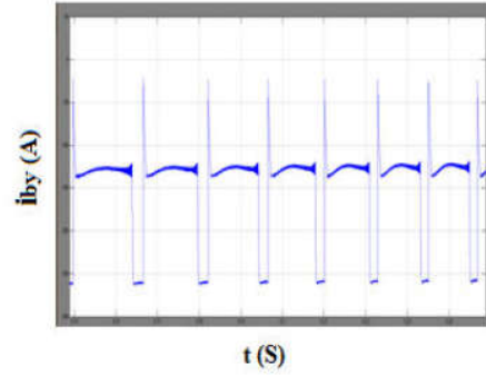
(a) Simulation results of driving-charging mode (mode 1)
