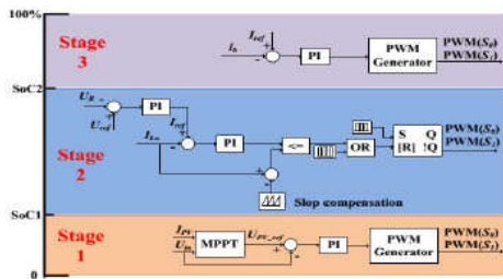
(c) Charging control strategy.
