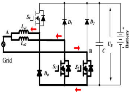
(c) Grid charging state 3 (Ugrid<0)
