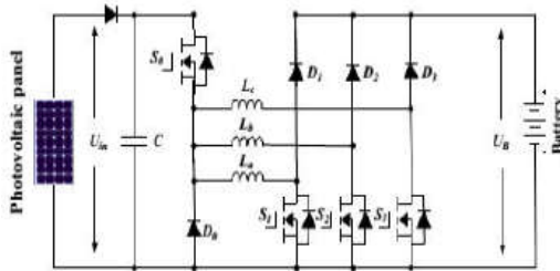
(a) Operation circuit under mode 1
