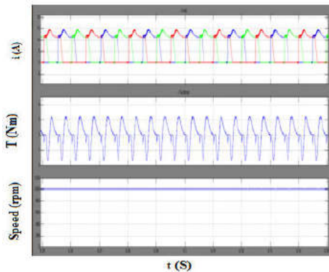
Fig27: Current, Torque and Speed
