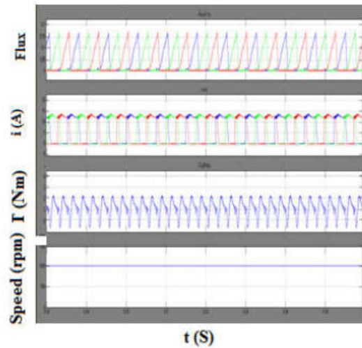
Fig23: Flux, Current, Speed and Torque
