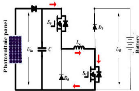
(a) Phase inductance charging
