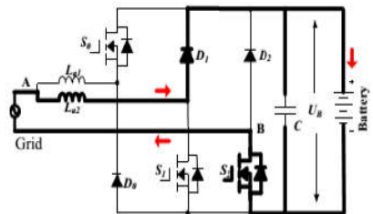
(b) Grid charging state 2 (Ugrid>0)
