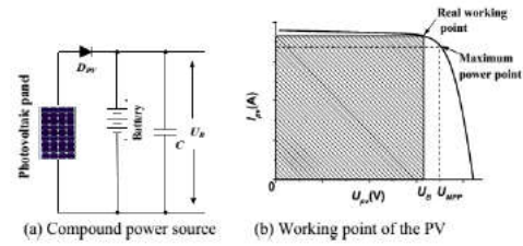
Fig6: Power supply at mode 2
