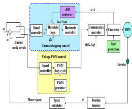
Fig8: SRM control strategy under single source driving mode
