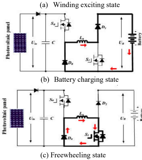
Fig9: Mode 1 working states
