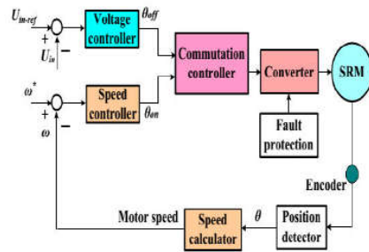
Fig10: Control strategy under driving-charging mode (mode 1)
