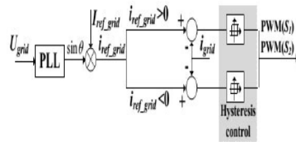
Fig12: Grid-connected charging control (Mode 5)
