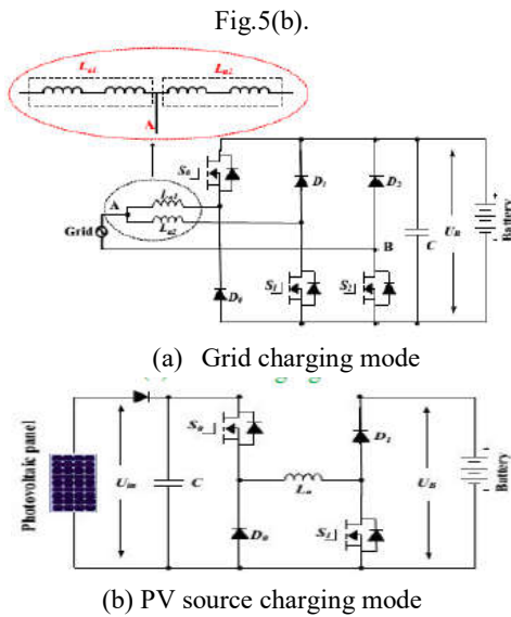
Fig5: Equivalent circuits of charging condition modes
