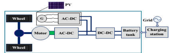
Fig1: PV-fed hybrid electrical vehicle
