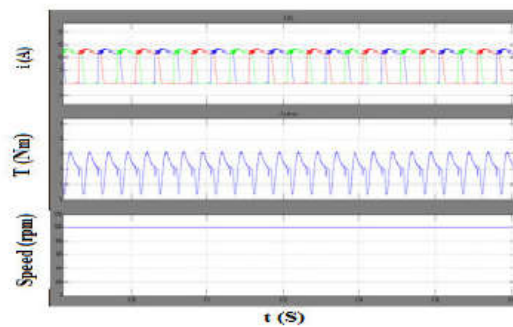
Fig25: Current, Speed and Torque
