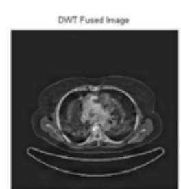
Figure4:DWT
