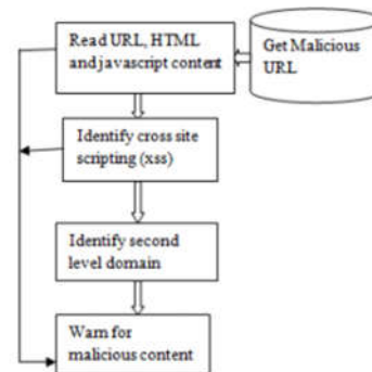
Figure.1. proposed methodology
