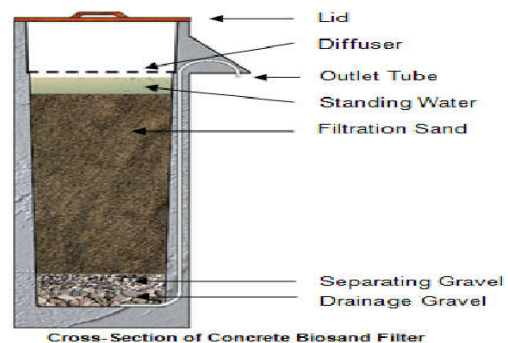
g. 1 Biosand Filtrations Process
