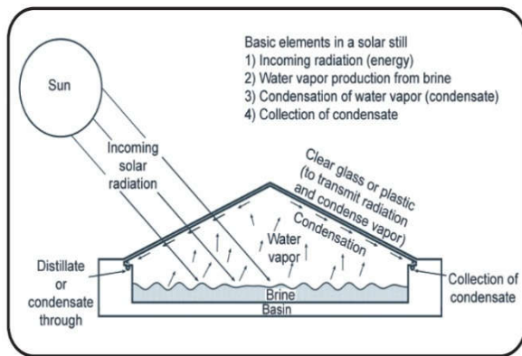
Fig. 2 Desalination Process
