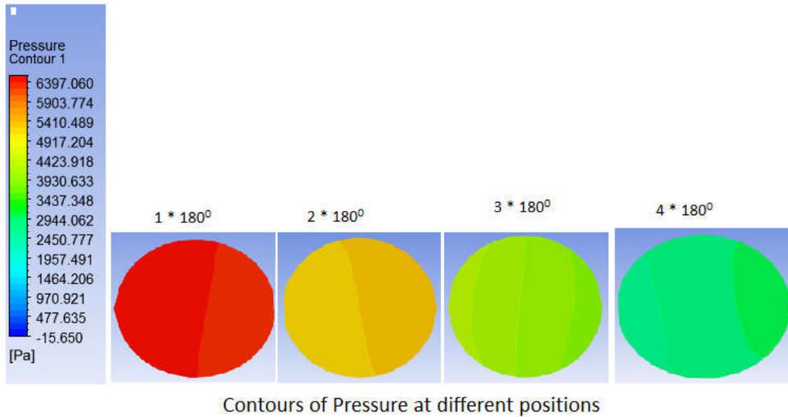
Fig.4.2 Contour plots of pressure at different positions, CFD – PBM model
