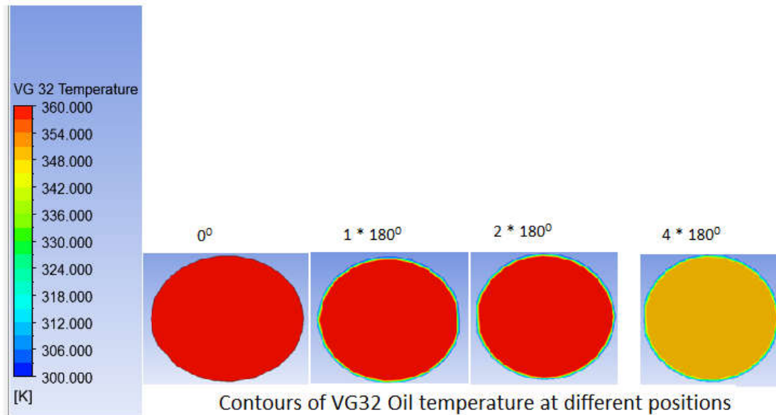
Fig 4.4 Contour plots of temperature of VG32 Oil at different position
