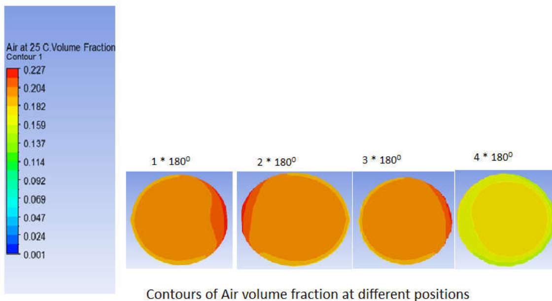
Fig.4.1 Contour plots of air volume fraction at different positions, CFD – PBM model
