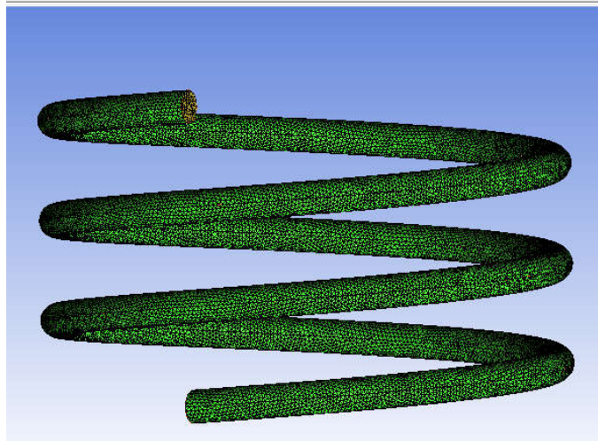
Figure .2. 3. Mesh generation for CFD simulations
