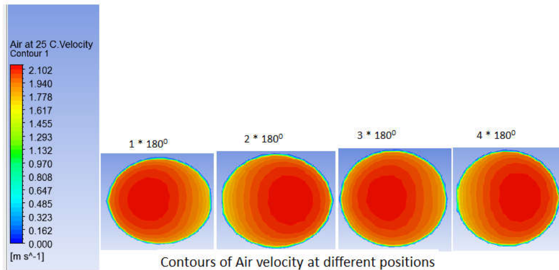
Fig.4.3 Contour plots of air velocity at different positions, CFD – PBM mode
