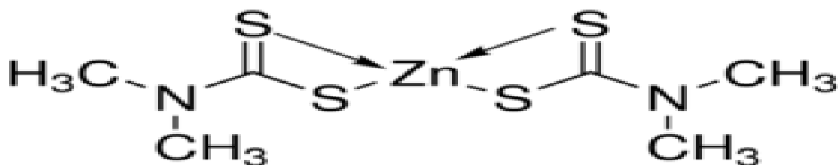
Structure of Ziram
