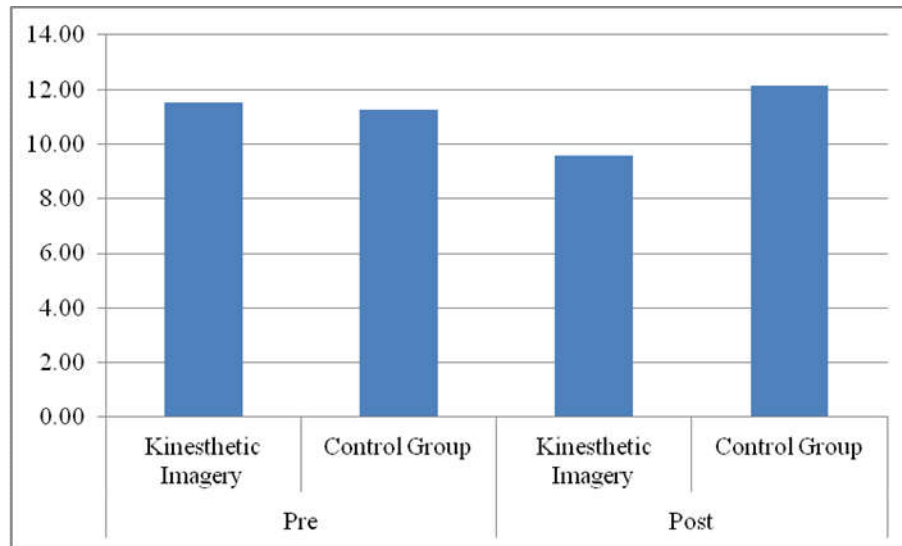
Figure 2: Mean hitting performance of Treatment and Control Group
