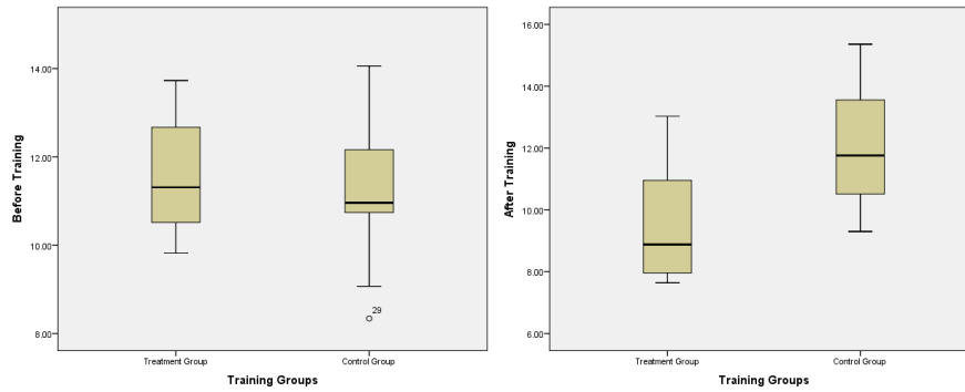
Figure 1: Box Plot test showing outliers
