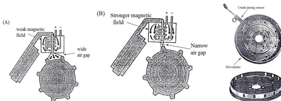
Fig.4.2.3 (A) Wide gap produces a weak magnetic field fig 4.2.3(B) Narrow gap produces a strong Magnetic field
