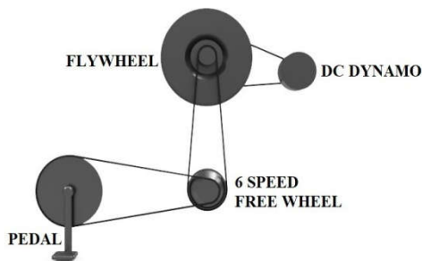
Fig 4 Schematic of transmission, front view
