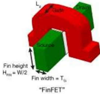
Fig 2: scaling of FinFET
