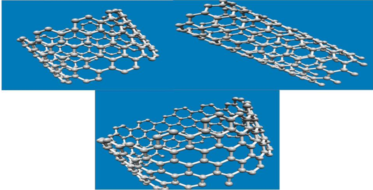
Fig.2. Nano tubes
