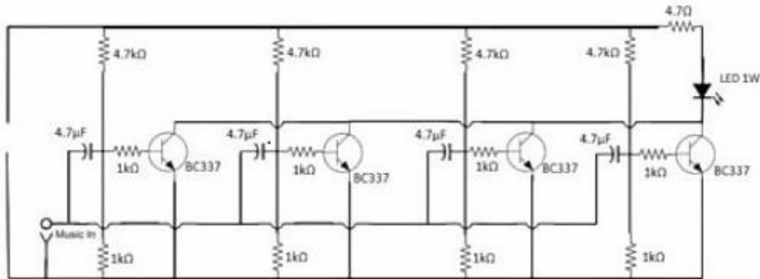
Fig 3.2.1 Transmitter circuit
