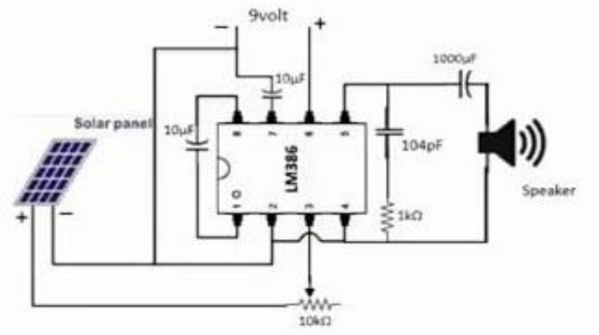
Fig 3.2.2 Reciver circuit
