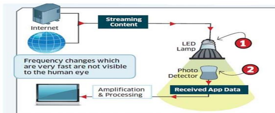
Fig 3.1.1 Block diagram
