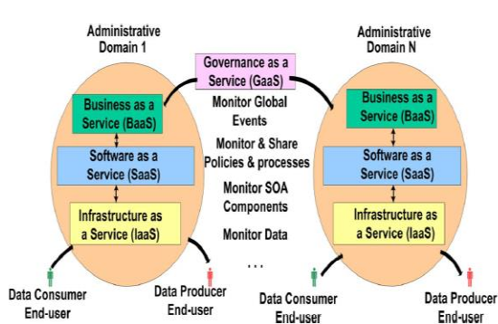
Fig.2. Net-centric SOA-based SoS.
