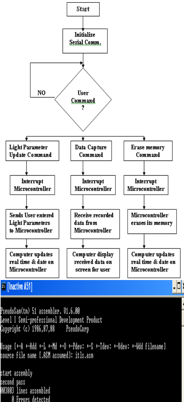
Figure 6 : Assembler GUI
